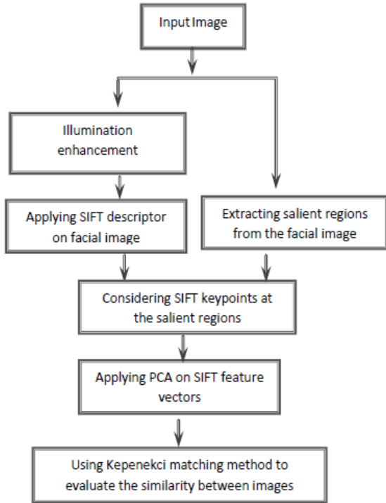
Figure 4. Flowchart of the Proposed Face Recognition System.
