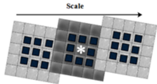
Figure 2. Showing Neighboring of a Pixel to Determine the Extrema Keypoints.
