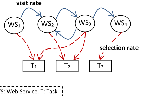
Figure 3. HMM Is Applied for the Service Selection Problem.
